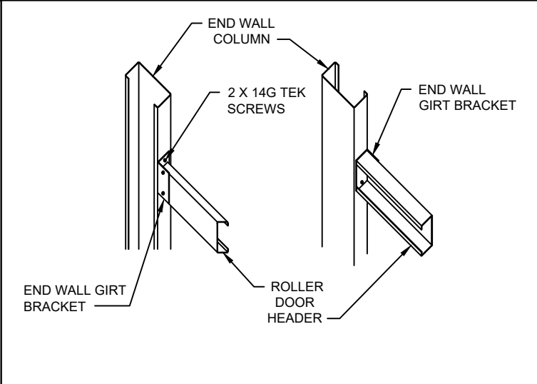
P END DOOR HEADER AND JAMB
