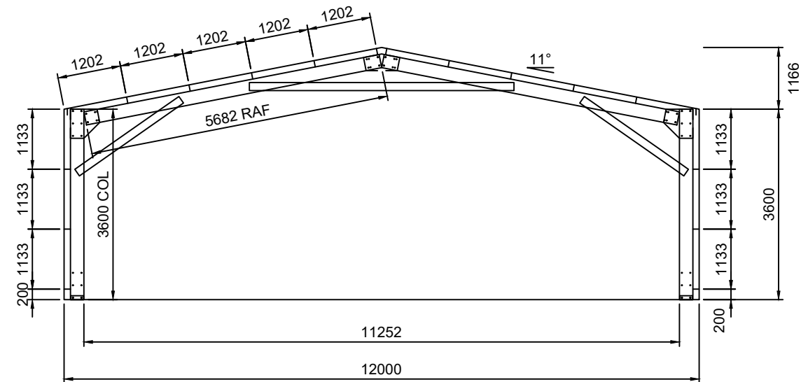
1 TYP. FRAME CROSS-SECTION 7 SCALE: 1:100 FRAMES 2-4
