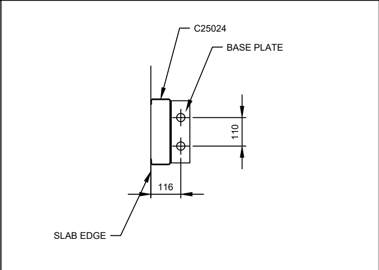
N ROTATED ENDWALL MULLION BASE
