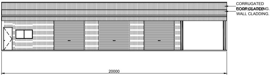
1 SIDEWALL EXTERIOR ELEVATION 7 SCALE: 1 = 200
