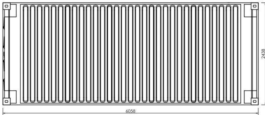
20ft Shipping Container - Roof Plan
