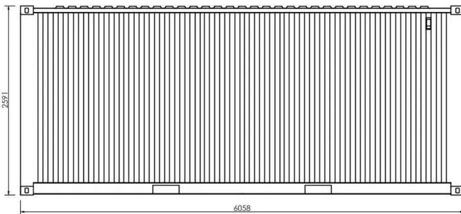
20ft Shipping Container - Side Elevation
