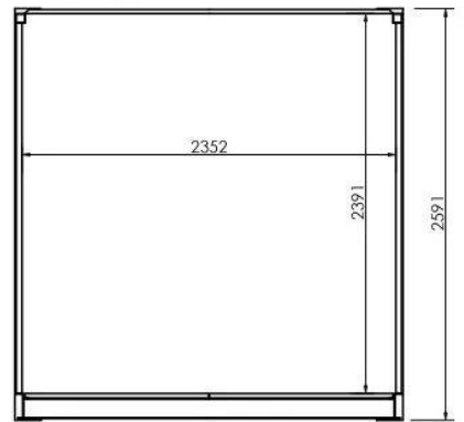
20ft Shipping Container - Section
