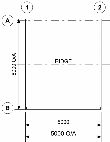
FRAME ROOF PLAN
