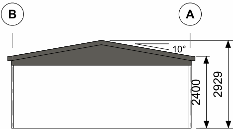
ELEVATION GRID 2
