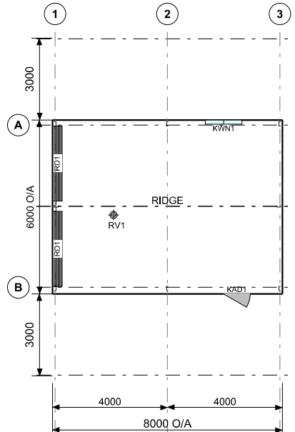
FRAME ROOF PLAN
