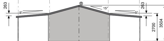
ELEVATION GRID 3
