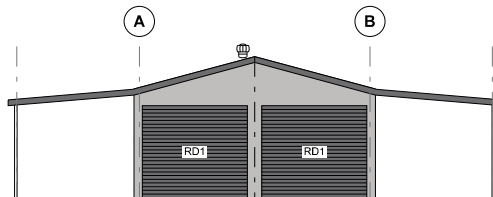
ELEVATION GRID 1
