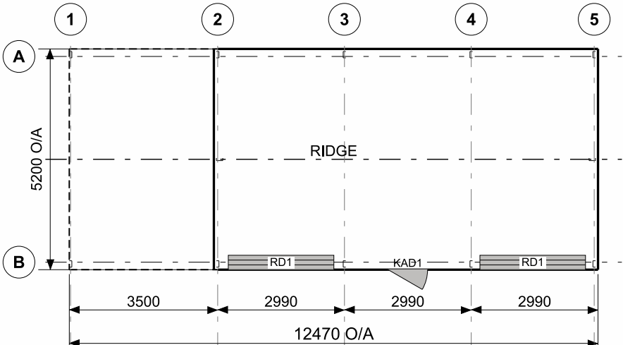
FRAME ROOF PLAN
